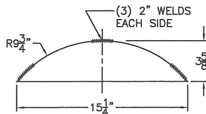
S.S. BAFFLE DETAIL
