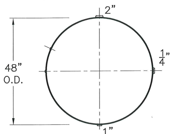
VIEW W/O SUPPORTS
