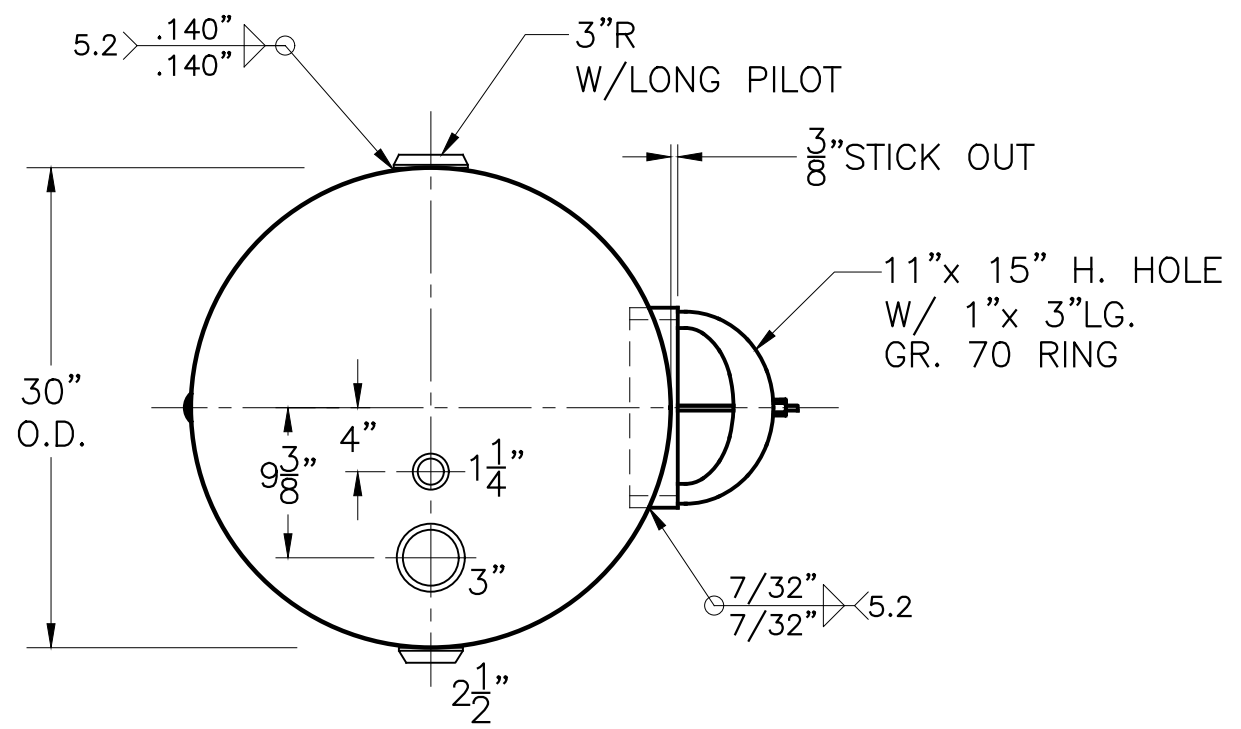
VIEW W/O SUPPORTS
