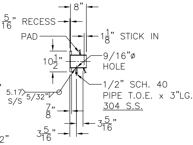
6" COLLAR DTL.
