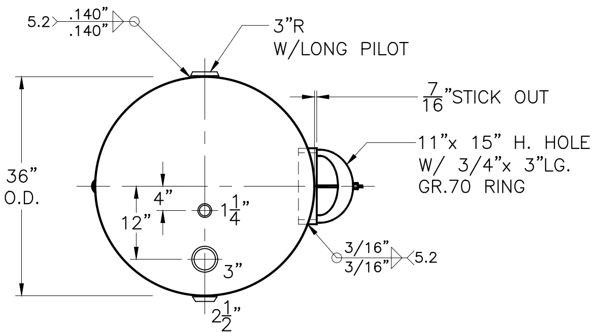
END VIEW W/O SUPPORTS
