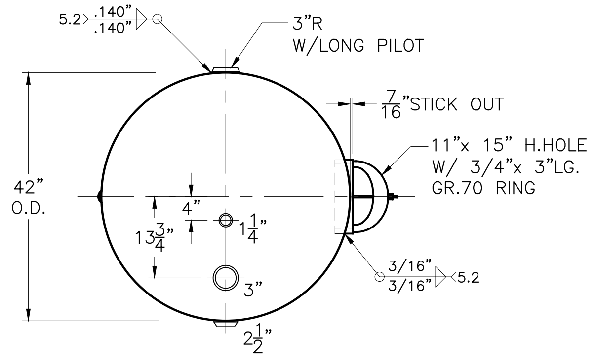
END VIEW W/O SUPPORTS
