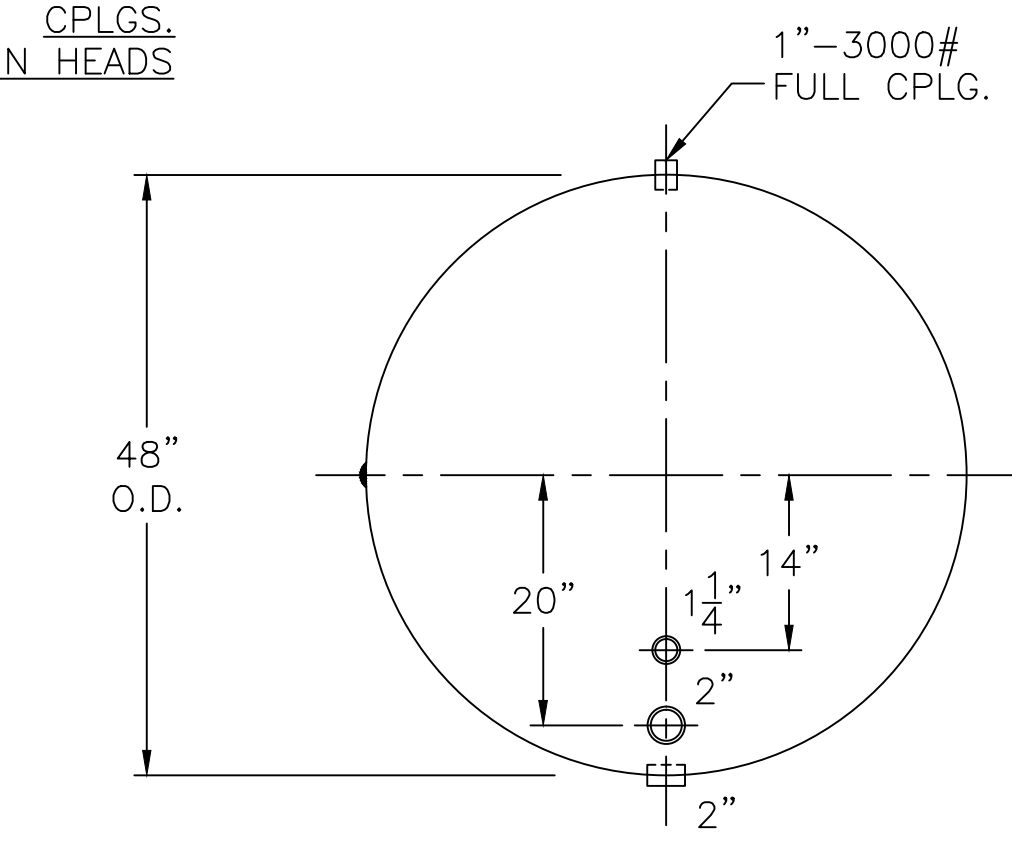
END VIEW W/O SUPPORTS
